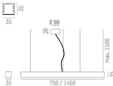
RIDE RING PD Massskizze 750 / 1450mm
