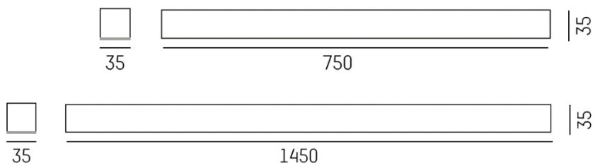
RIDE RING SD Massskizze 750 / 1450mm
