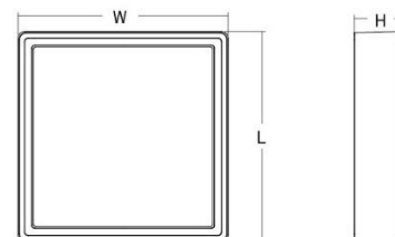
CAZIS SQUARE: L 240 x B 240 x H 77mm
